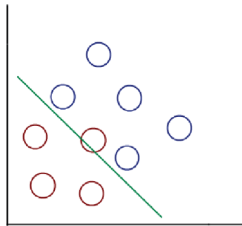
Figure 2. Geometrical Interpretation of SOC Constraint
