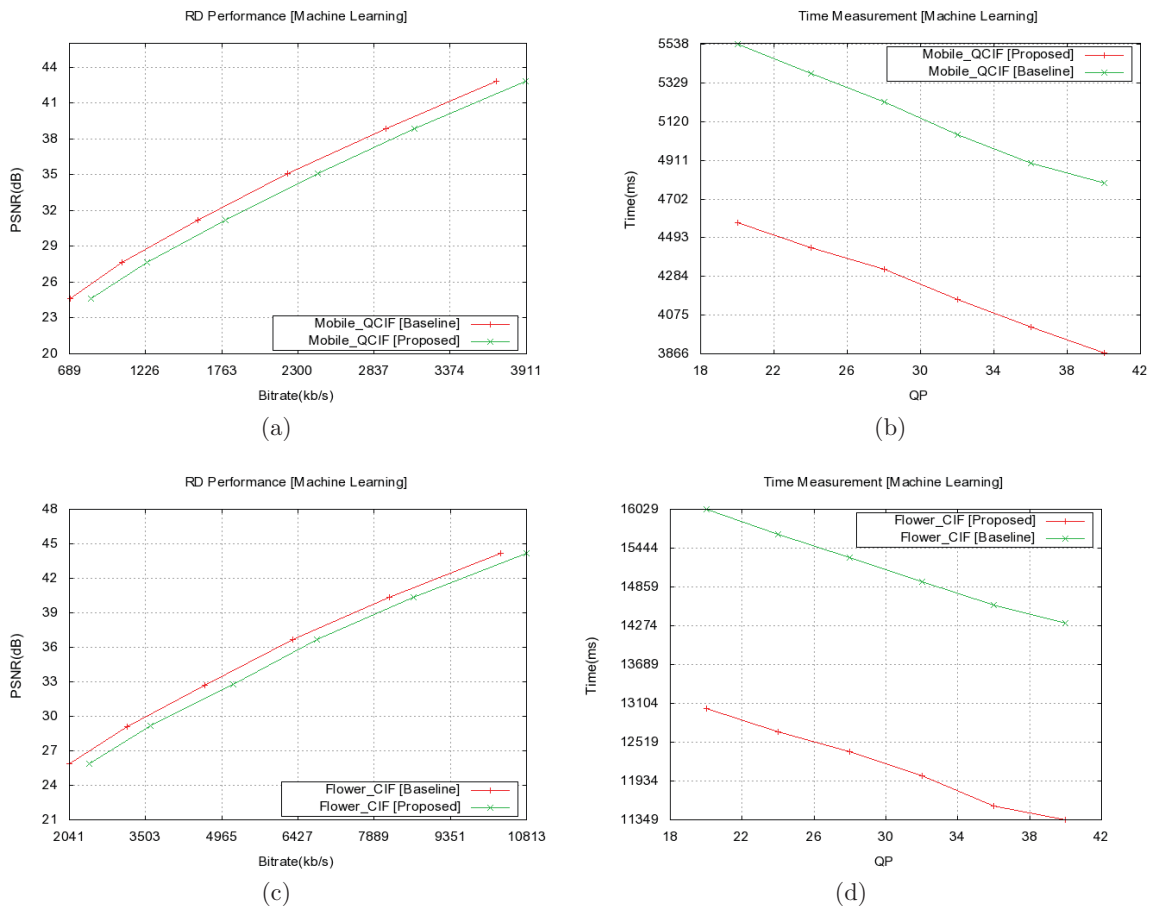
Figure 5. (a)(c) RD performance of the H.264 Intra frame encoder with Machine Learning classifier; (b)(d)Time complexity reduction.
