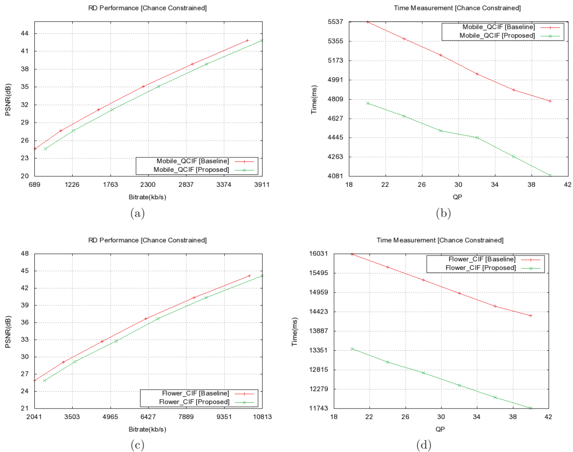
Figure 4. (a)(c) RD performance of the proposed H.264 Intra frame encoder with Chance Constrained classifier; (b)(d)Time complexity reduction.
