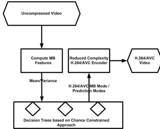
Figure 1. Applying chance constrained classifier in video coding
