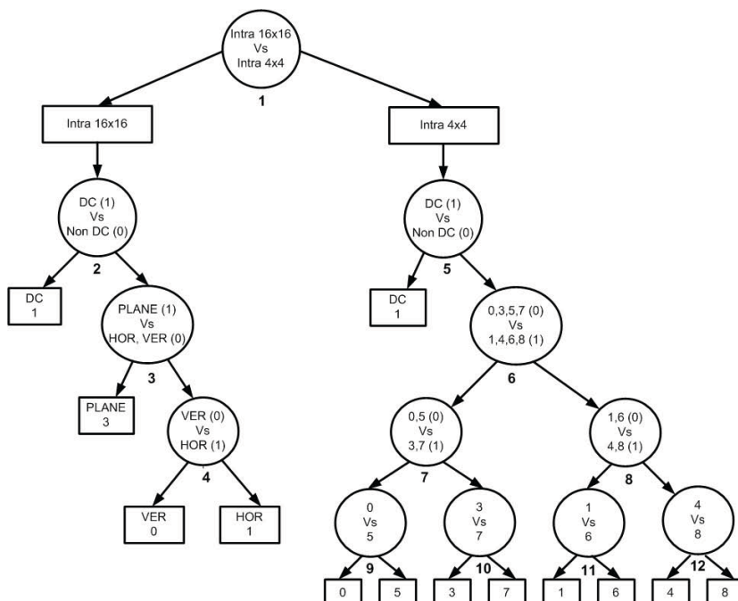
Figure 3. Decision tree used in Intra MB coding
